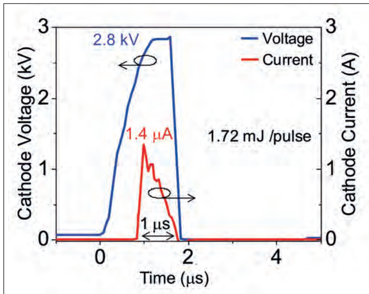
► Figure 3. Current and voltage waveforms of a 3 kV GaN vertical p-n diode during avalanche breakdown. The diode voltage clamps and a high current flows from cathode to anode in avalanche mode.
