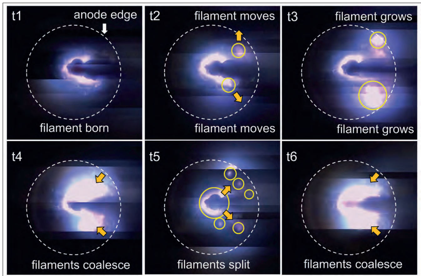
► Figure 5. Top view optical images of a GaN vertical p - n diode at different instants during an avalanche breakdown. A high voltage, unclamped inductive switching pulse train applied to the diode pushes it into the avalanche breakdown mode. At breakdown, current filaments (or micro-plasma tubes) form which later dynamically move around, spreading the heat across the diode area as the avalanche progresses.
