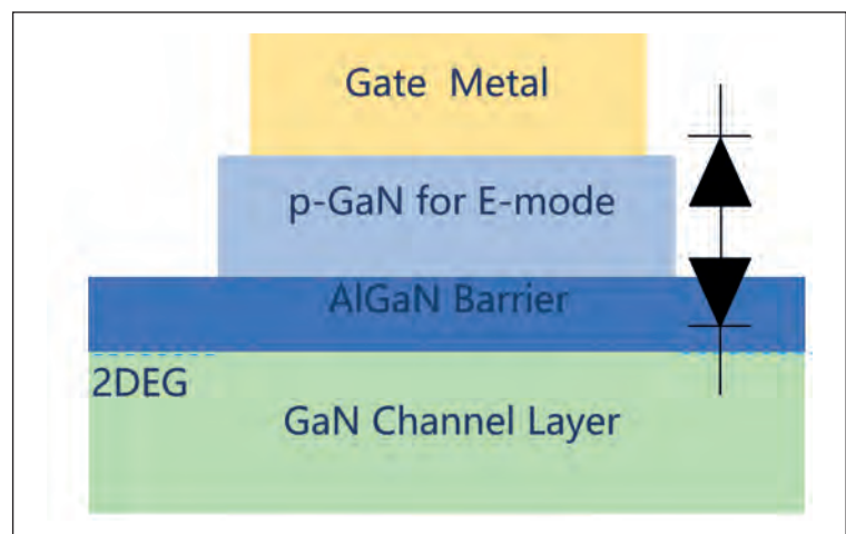
➤ Figure 3: The inherent back-to-back diodes in the gate structure require that strict process control be implemented to achieve leakage under 3 μA at 85°C for BiGaN.
