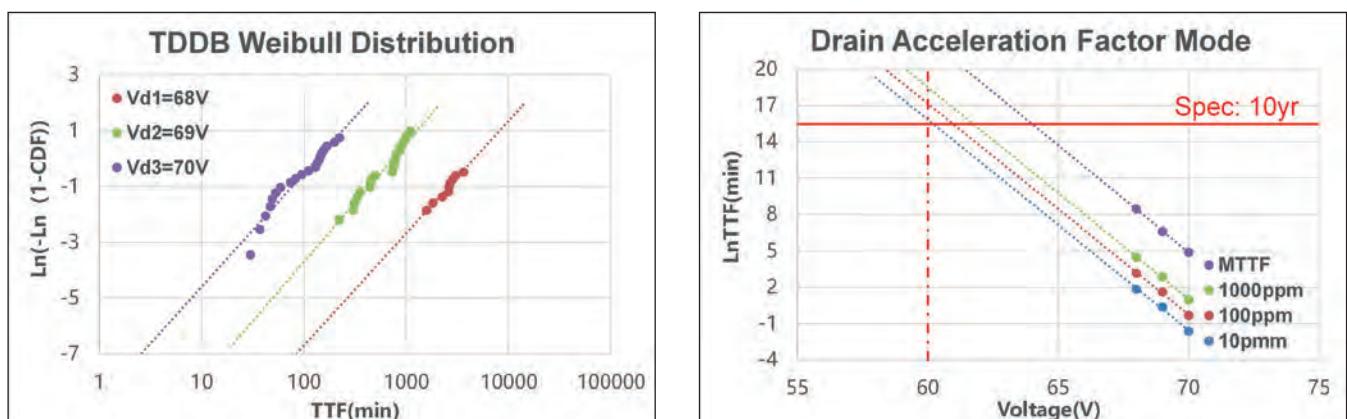
➤ Figure 5: BiGaN Drain robustness: a) TDDDB Weibull distribution; b) Drain acceleration mode.
