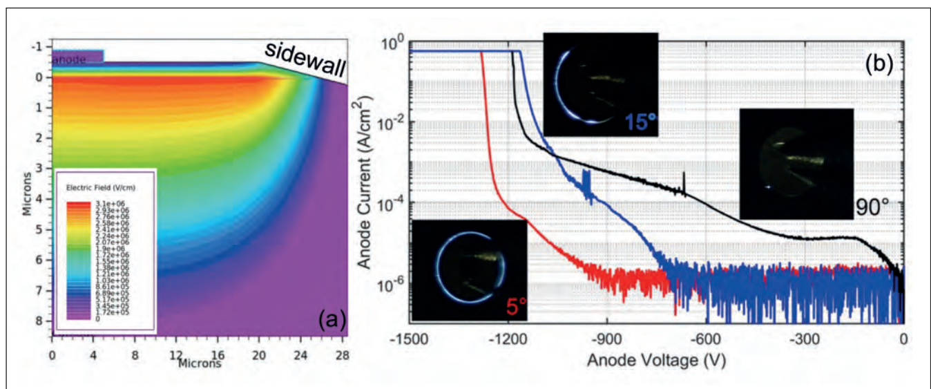
► Figure 2. Avalanche breakdown study for a 1.2 kV GaN vertical p - n diode. (a) Bevel termination redistributes the electric field, triggering avalanche mechanism in the bulk GaN. (b) Reverse characteristic of the diode studied at different bevel angles. A uniform electroluminescence (light emission) occurs at breakdown in the diode with a 5^\circ angle, exhibiting 1.2 kV avalanche breakdown voltage.
