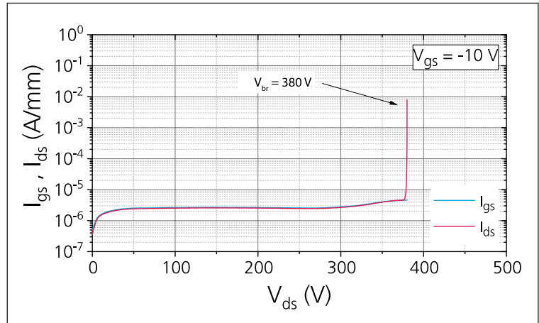
➤ Figure 1. Drain-Source breakdown characteristics for a device with a total gate width of 1.2 mm (6 x 200 \mu\text{m} ). For the measurement, the source of the device is grounded, whereas the gate potential is set to -10 V. Then the drain potential is quickly raised until the recorded gate and drain current exceed the compliance value of 1 mA/mm, which is considered as breakdown.
