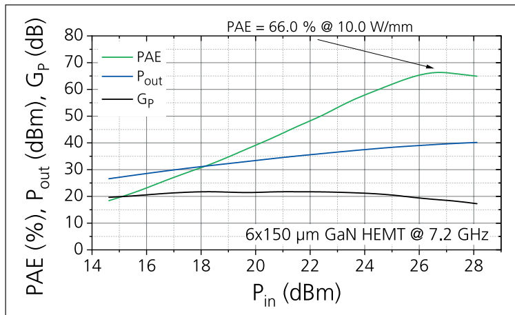
➤ Figure 4. Pulsed load-pull measurements of a 100 V GaN HEMT with a total gate width of 0.9 mm (6 x 150 \mu\text{m} ) at 7.2 GHz. The pulse width is 100 \mu\text{s} , with a duty cycle of 10 percent. For this measurement a ‘trade-off’ of fundamental impedance was chosen that yielded a good combination of efficiency and power density. Additionally, the second harmonic at the output of the device was set for the value that showed the highest power-added efficiency.
