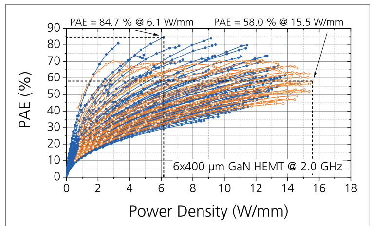
➤ Figure 2. Pulsed load-pull measurements of a 100 V GaN HEMT with a total gate width of 2.4 mm (6 x 400 \mu\text{m} ) at 2.0 GHz. The pulse width is 100 \mu\text{s} with a duty cycle of 10 percent. Two conditions are plotted here. Orange is for load pull at the fundamental frequency without termination of harmonics, while blue is for fundamental load pull with second harmonic impedances at input and output set for maximum efficiency.
