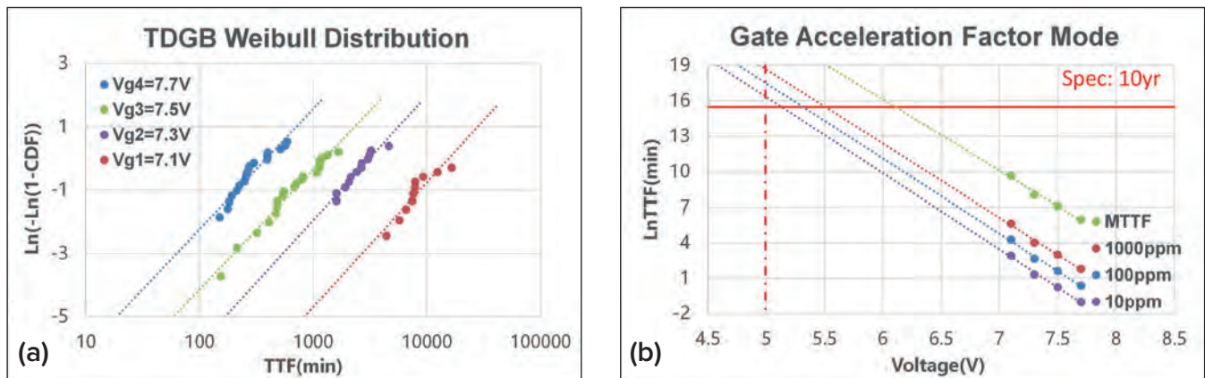
➤ Figure 4: BiGaN Gate robustness: a) TGDB Weibull distribution; b) Gate acceleration mode.
